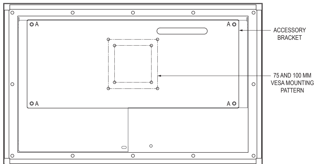
FIGURE 1 – REAR VIEW OF ML19.5 MONITOR (FACE DOWN)
