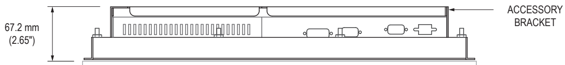
FIGURE 2 – BOTTOM VIEW
