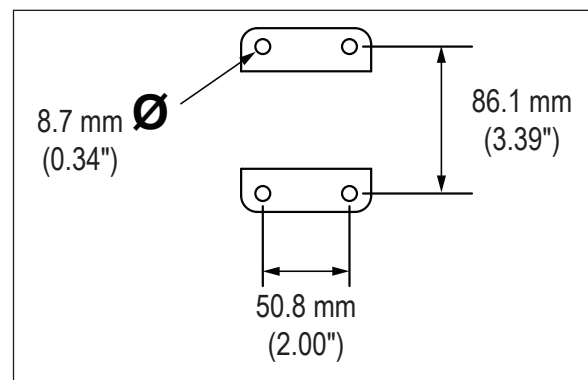
FIGURE 1 – YA __ -15- __ MOUNTING PATTERN
