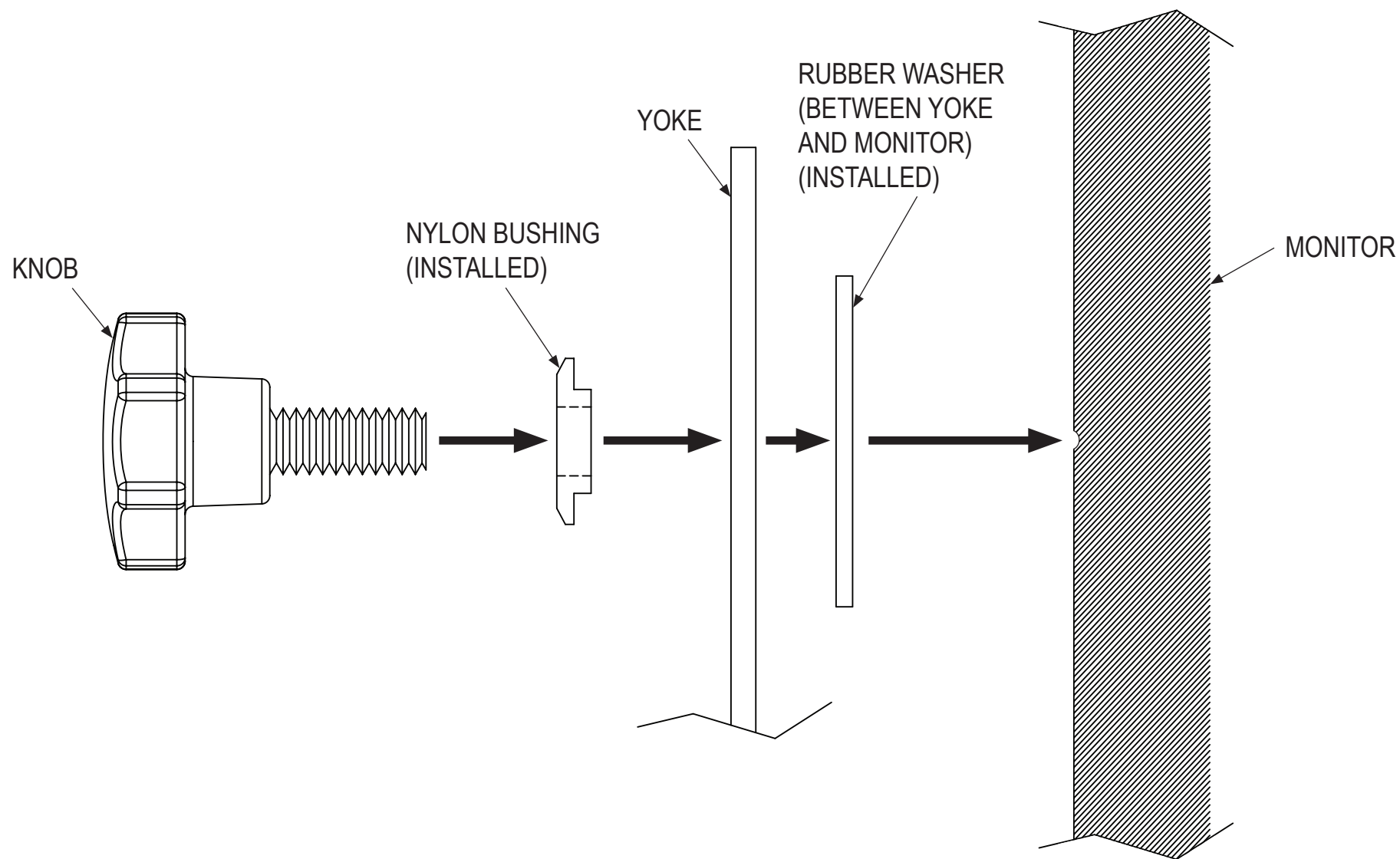
FIGURE 3 – YOKE MOUNTING HARDWARE
