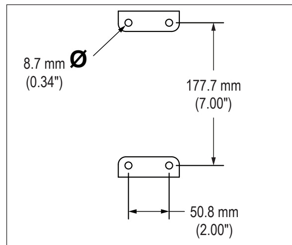
FIGURE 2 – YA __ -24- __ MOUNTING PATTERN
